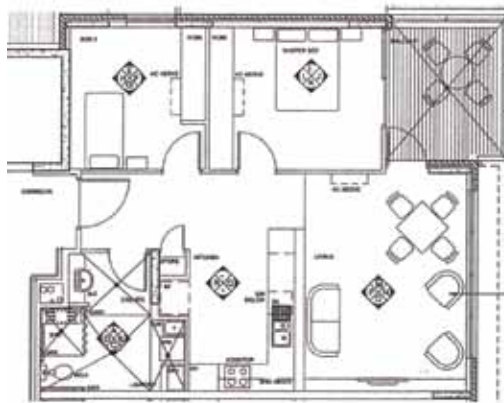
01 2 BEDROOM UNIT TYPICAL A102 MAIN 3 STOREY BUILDING
