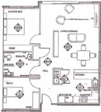
01 2 BEDROOM ILLU No. 1,2,3,4,5 & 6 TYPICAL A102 SINGLE BUILDINGS
